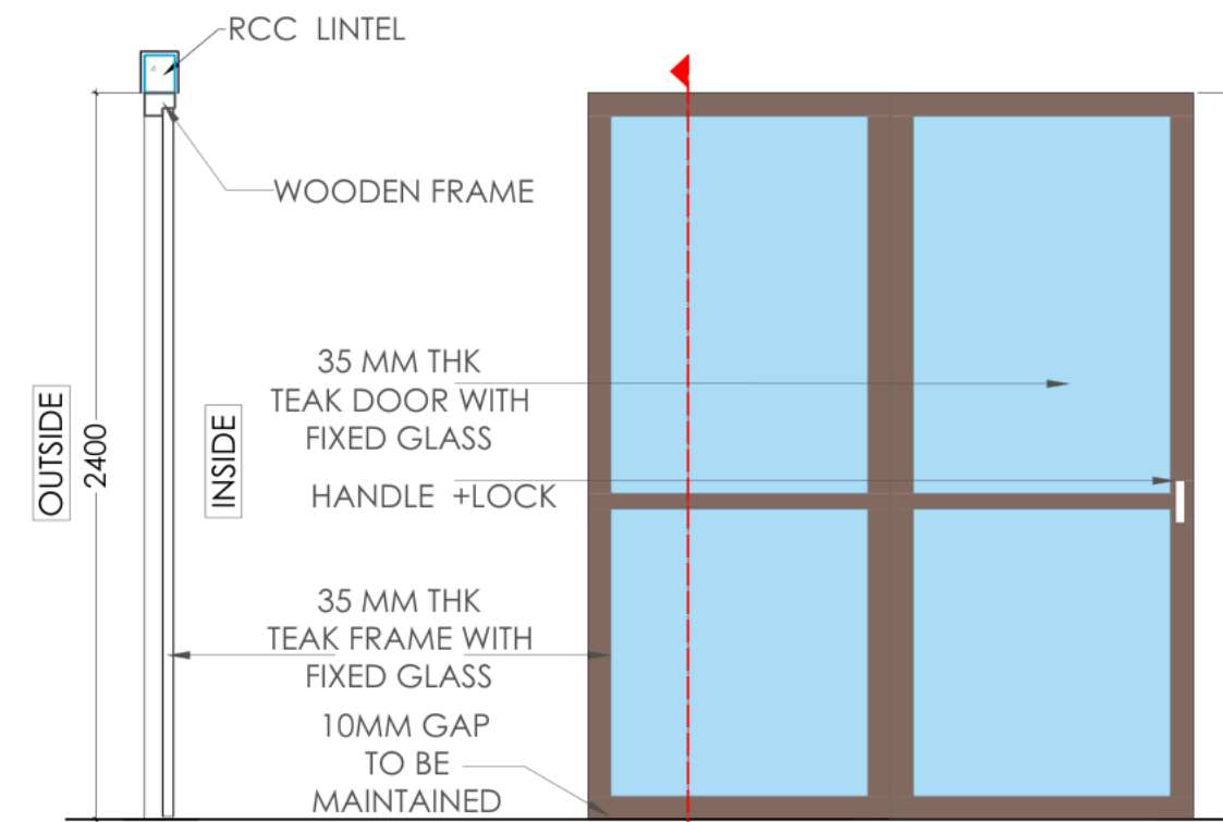
SECTION ELEVATION
