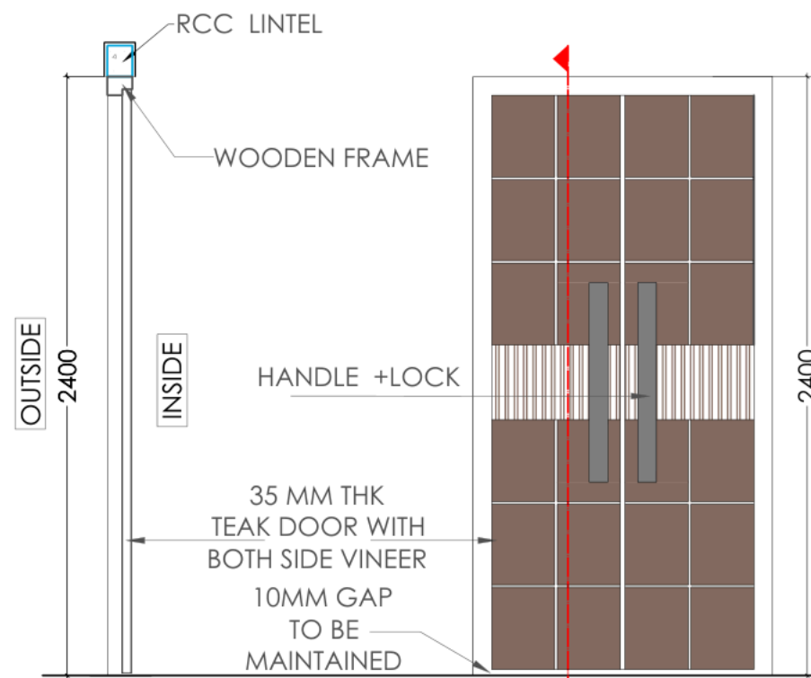
SECTION ELEVATION
