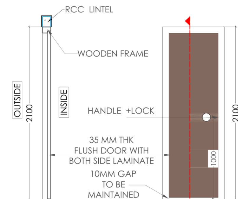
SECTION ELEVATION
