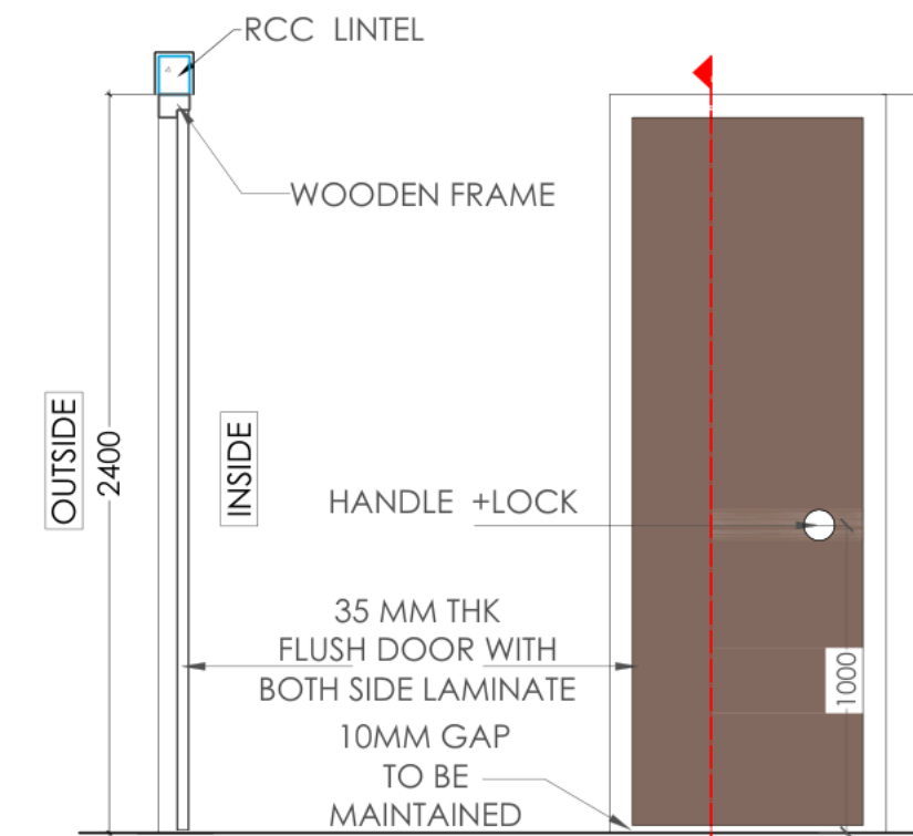
SECTION ELEVATION
