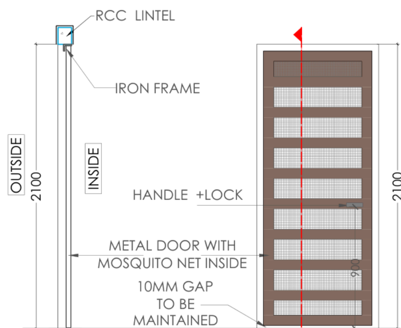
SECTION ELEVATION
