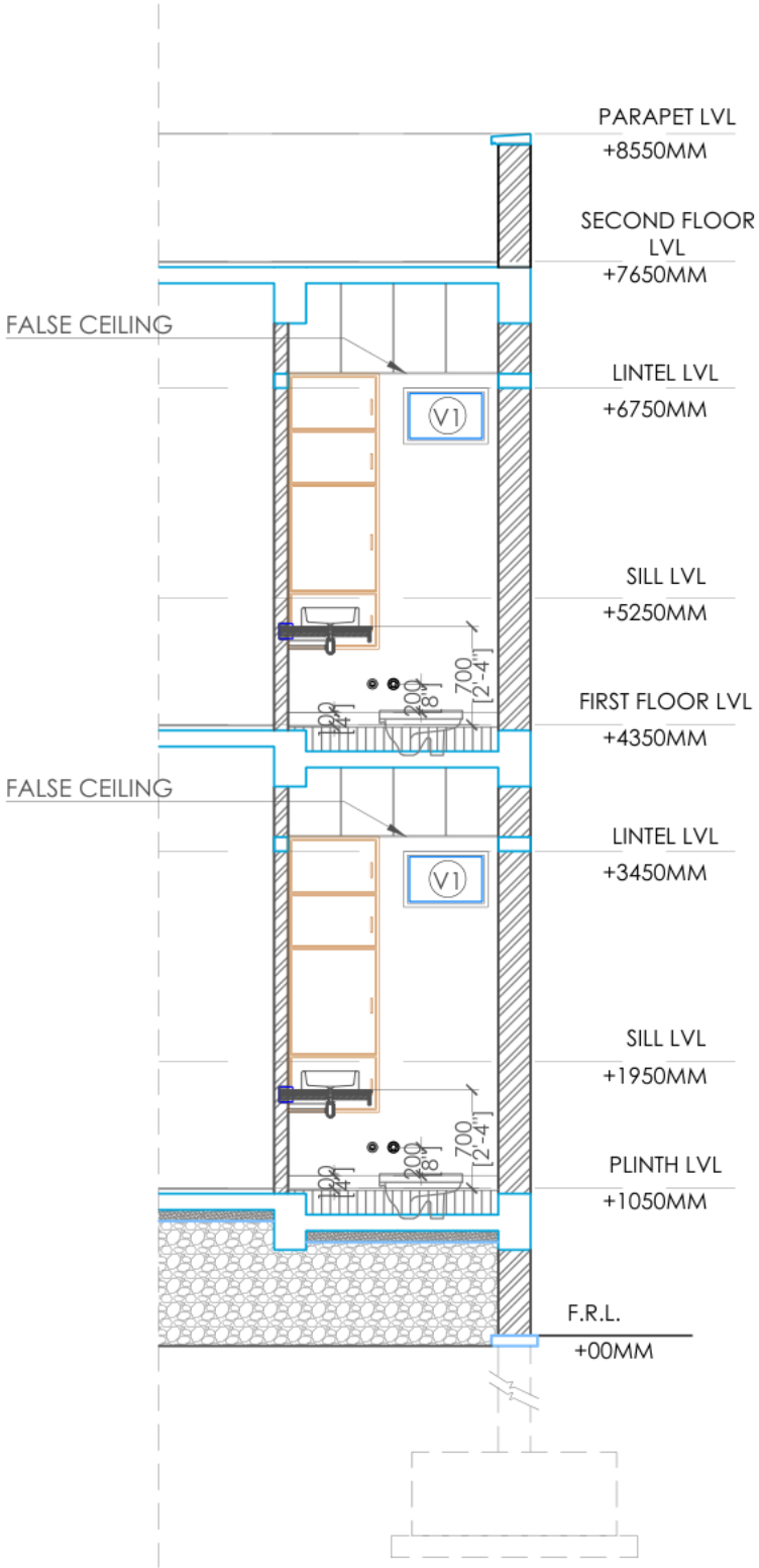
SECTION E-E'
