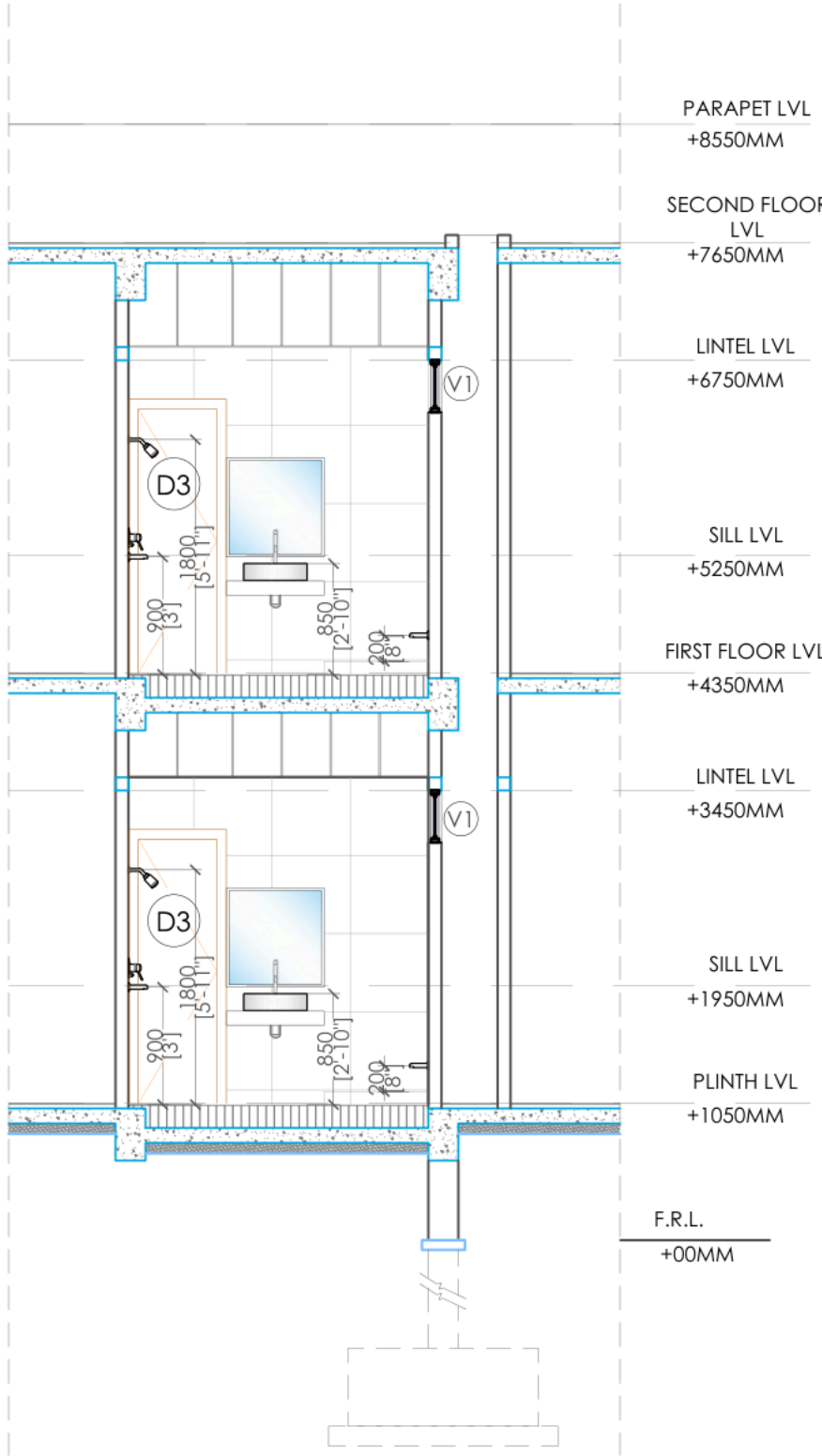
SECTION X-X'
