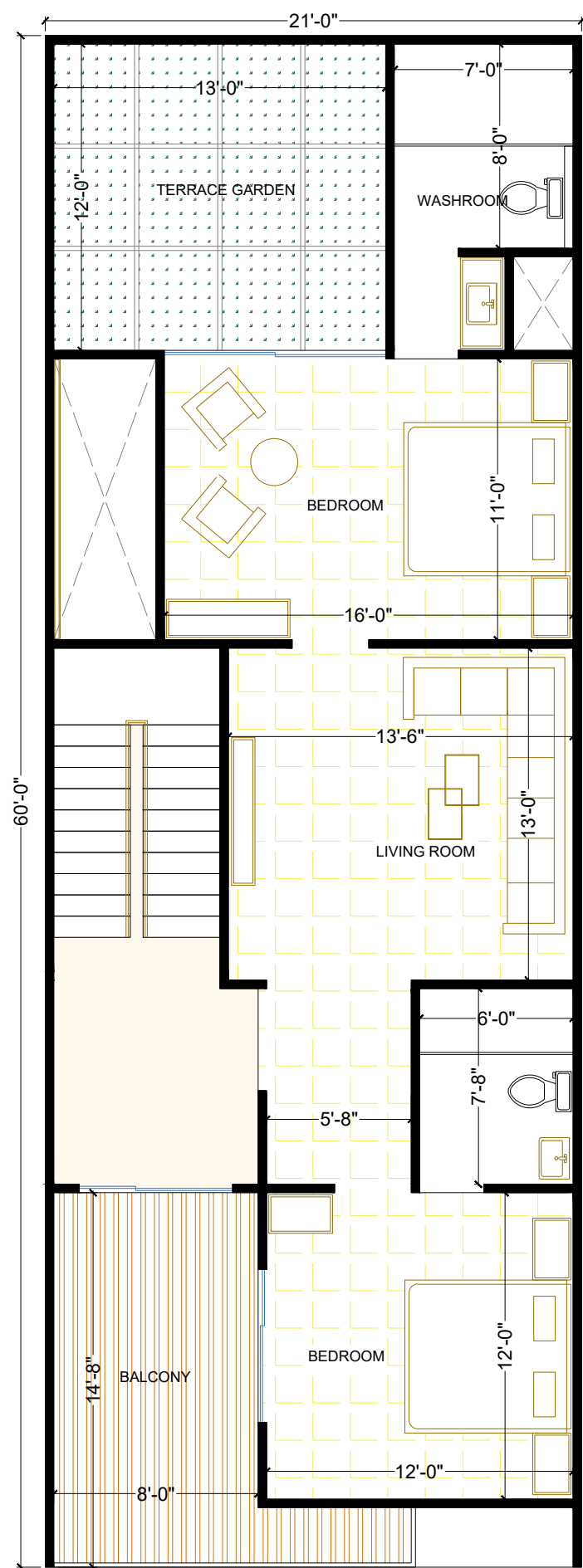
FIRST FLOOR
